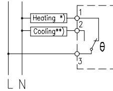
TRW 60 / TKW 60 Changeover contact (CO)
