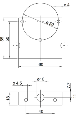
Mounting bracket 6401
