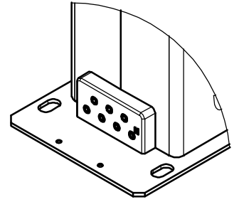
Secondary terminal's detail
