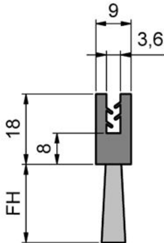
For sheet metal thickness 1.5 - 2 mm All dimensions in mm
